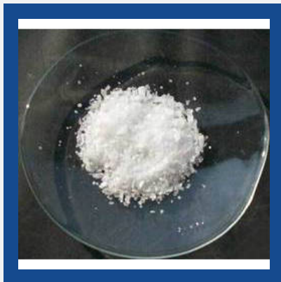
Boric Acid
