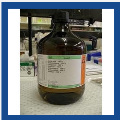
Acetic Acid
