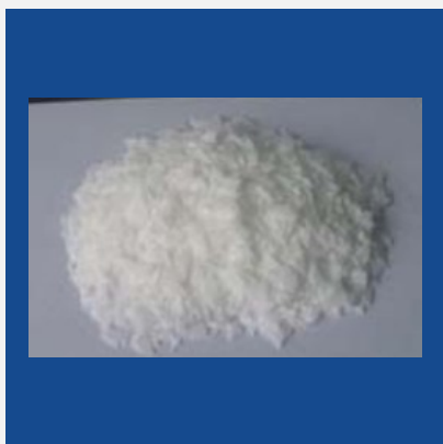
Phthalic Anhydride
