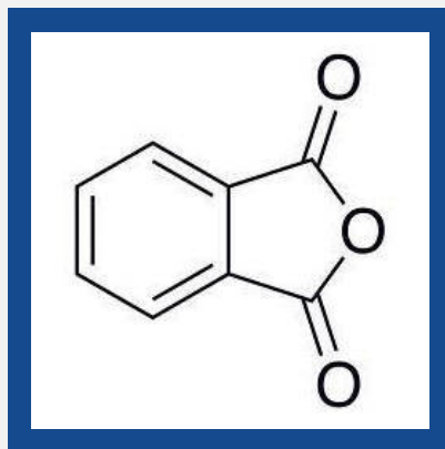
Phthalic Anhydride
