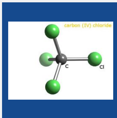
Carbon Tetrachloride
