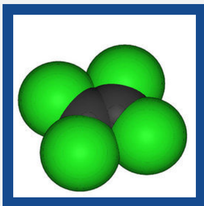
Perchloroethylene
