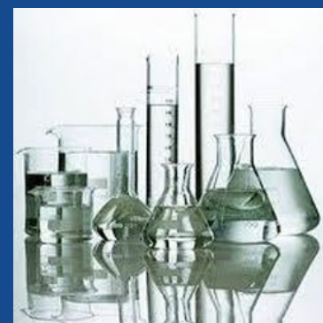
Diethylene Glycol
