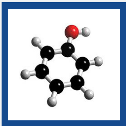
Phenol
