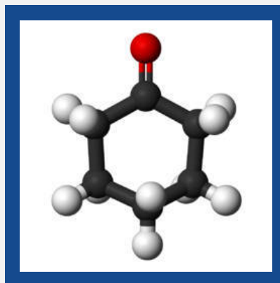
Cyclo Hexanone
