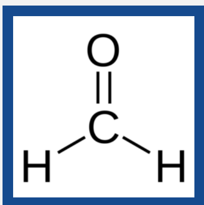
Formal Dehyde
